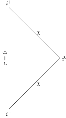
Figure 23: Penrose Diagram for Minkowski space
