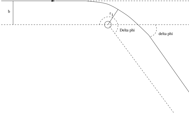
Figure 15: Bending of light by a star. Indicated are the definitions of the impact parameter b , the perihelion r_1 , and of the angles \Delta\phi and \delta\phi .
